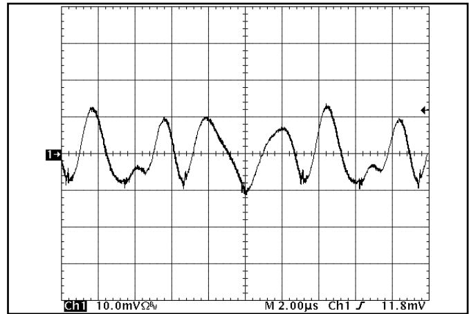
Figure 14: Input reflected ripple current, i_s , through a 10\mu\text{H} source inductor at nominal input voltage and rated load current (20mA/div). See Figure 12.
