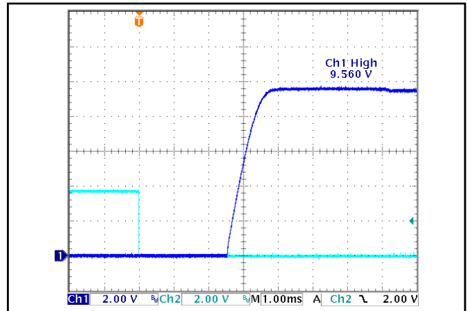
Figure 10: Turn-on transient at zero load (1.0 ms/div). Top Trace: V OUT (2V/div). Bottom Trace: ON/OFF input (1V/div).
