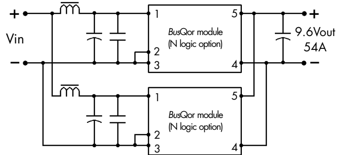
Figure H: BusQor Output Paralleling for increased current output.
