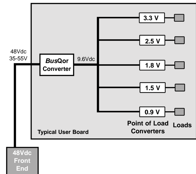
Figure A: Example of Intermediate Bus Architecture using BusQor bus converter and point of load non-isolated converters
