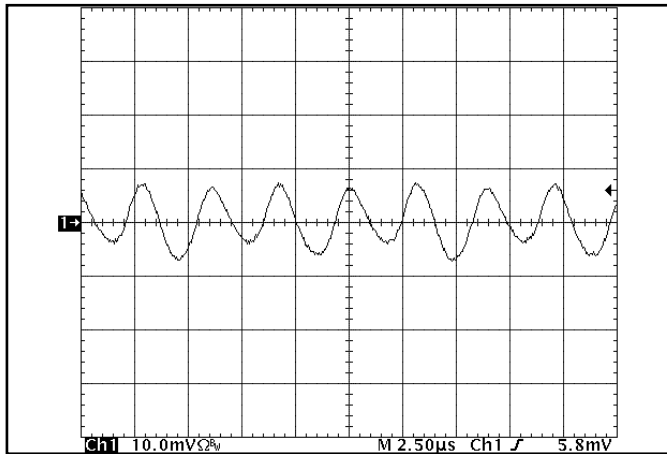
Figure 13: Input Terminal Ripple Current, i_c , at full rated output current and nominal input voltage with 10\mu\text{H} source impedance and 47\mu\text{F} electrolytic capacitor (500 mA/div). See Figure 12.
