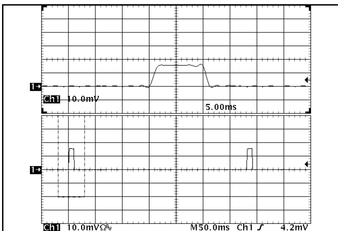
Figure 17: Load current (50A/div) as a function of time when the converter attempts to turn on into a 1\text{m}\Omega short circuit. Top trace (5.0ms/div) is an expansion of the on-time portion of the bottom trace.
