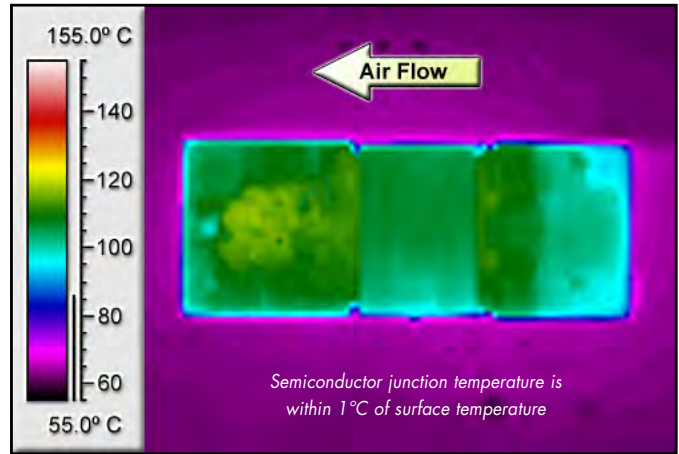
Figure 8: Thermal plot of converter at 27 amp load current (250W) with 55°C air flowing at the rate of 200 LFM. Air is flowing across the converter from output to input (nominal input voltage).
