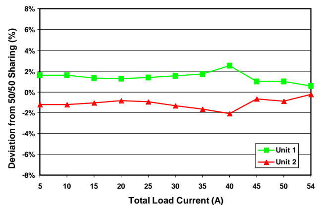
Figure K: Current share performance of 2 paralleled modules
