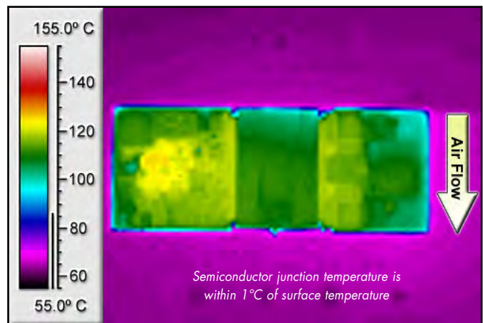
Figure 6: Thermal plot of converter at 27 amp load current (250W) with 55°C air flowing at the rate of 200 LFM. Air is flowing across the converter from pin 1 to pin 3 (nominal input voltage).
