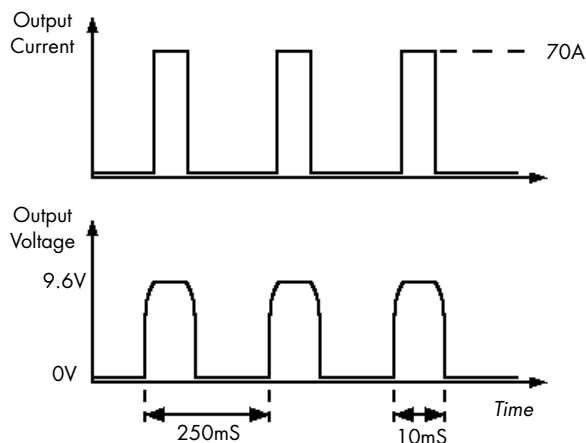
Figure D: Output Short Circuit and Auto-Resetting protection diagram (not to scale)
